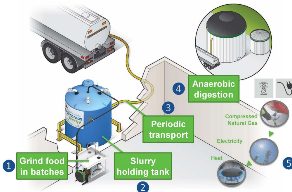
Figure C-1. Grind2Energy Process.
